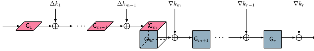
Figure 2: The BC in the related-key setting for a composite key-alternating cipher F = F_r \circ \dots \circ F_{m+1} \circ F_m \circ \dots \circ F_1 .
