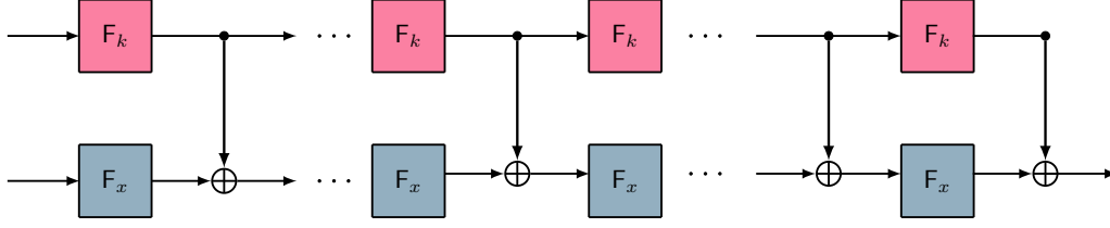
Figure 9: The key-alternating cipher.
