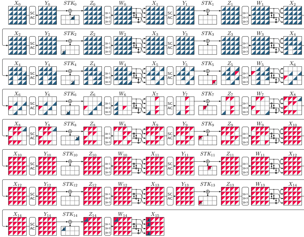
Figure 5: 15-Round boomerang distinguisher for SKINNY-64-192 from the tool in [HBS21].
