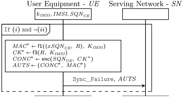
Fig. 5. Fix F1: Fix by symmetrically encrypting SQN_{UE}
