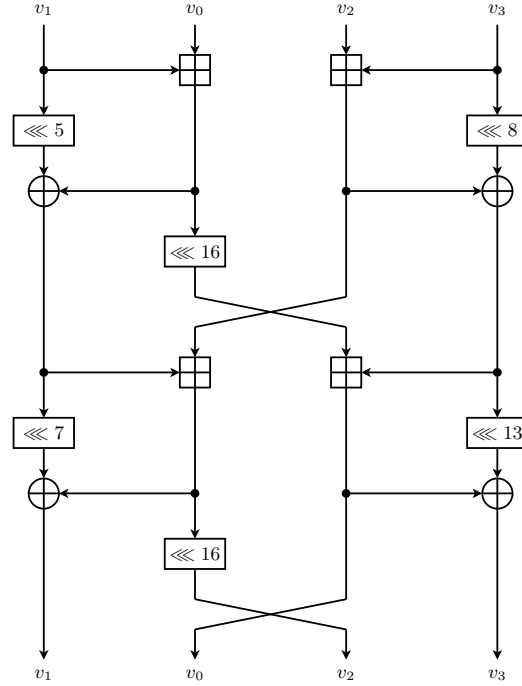
Fig. 2. A round of the Chaskey permutation \pi , defined as: v_0 \| v_1 \| v_2 \| v_3 \leftarrow \pi(v_0 \| v_1 \| v_2 \| v_3) . We intentionally swapped v_0 and v_1 , as this reduces the number of crossing lines in the figure.
