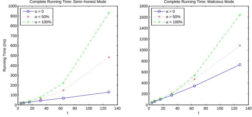
Fig. 5. Complete execution time. Left: Semi-honest mode. Right: Malicious mode.
