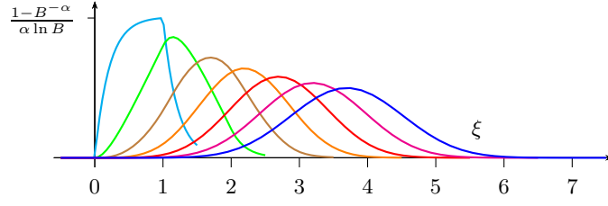
Figure 4.2: \tilde{\lambda}_{\text{norm}}^k(\xi) for \xi \in [-\frac{1}{2}, k + \frac{1}{2}] and k = 1, 2, 3, 4, 5, 6, 7
