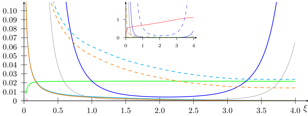
Figure 10.3: Errors of the various estimates relative to \tilde{\kappa}_{B,C}^k . Parameters are as in Figure 10.1.
