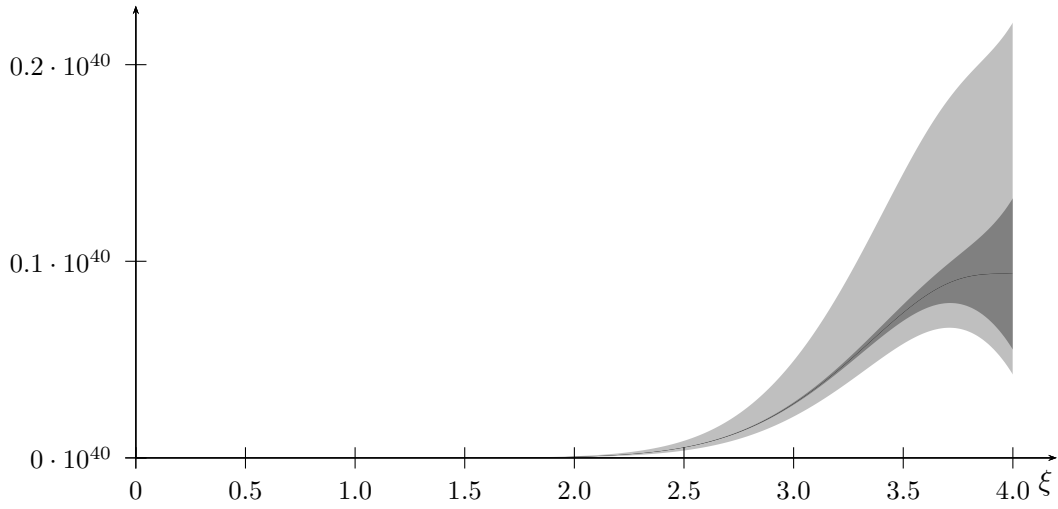
Figure 10.1: Absolute behavior of the estimates for \kappa_{B,C}^k(\xi) . The light gray area shows the \lambda estimate, the dark gray area the \eta estimate, and the black area (well, yes) shows the \kappa estimate. The parameters are B = 1100 \cdot 10^6 , C = 2^{37} - 1 , \alpha = \ln(C)/\ln(B) - 1 = 0.2327 , k = 4 .
