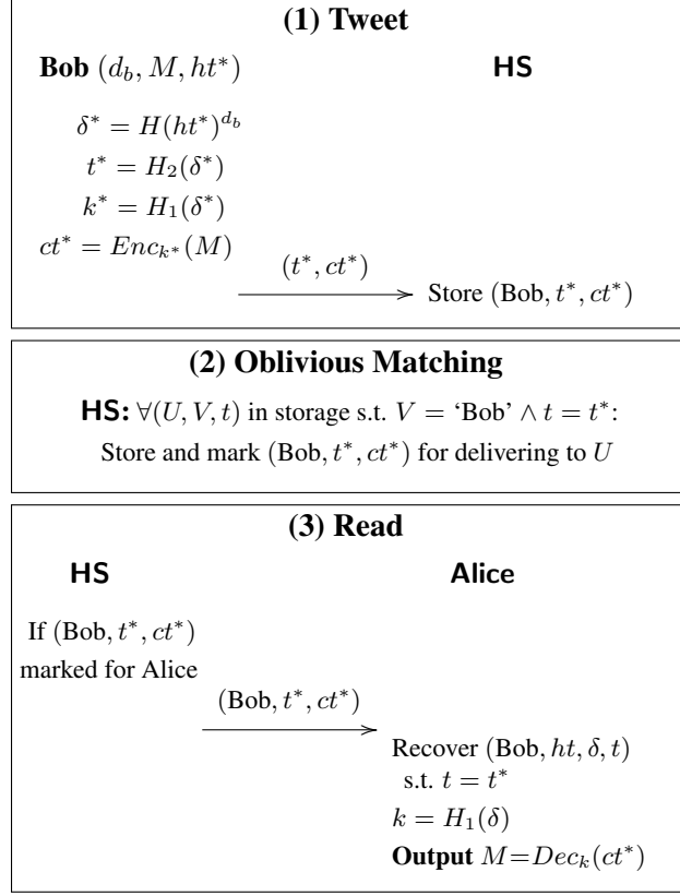
Figure 3: Tweeting and reading in Hummingbird. It executes on common input H, H_1, H_2 . All computation is mod N_b .
